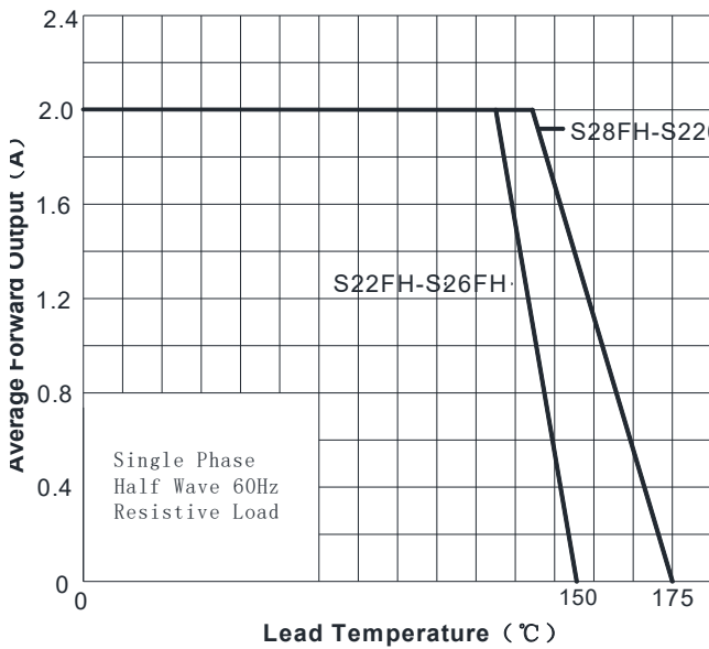
FIG1:Io-TL Curve
